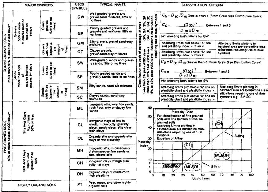
Figure 1-1. Unified soil classification system criteria 1-6
