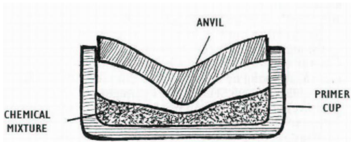
Cross section of Boxer primer.
