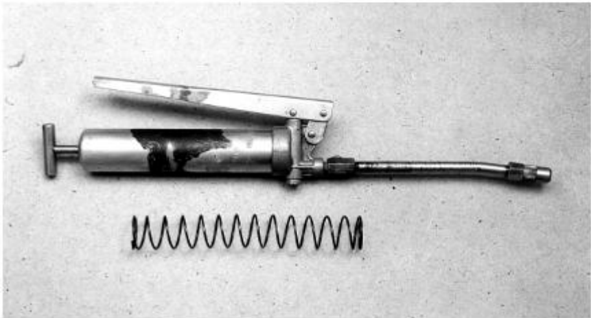
Side lever grease applicator and internal spring.
