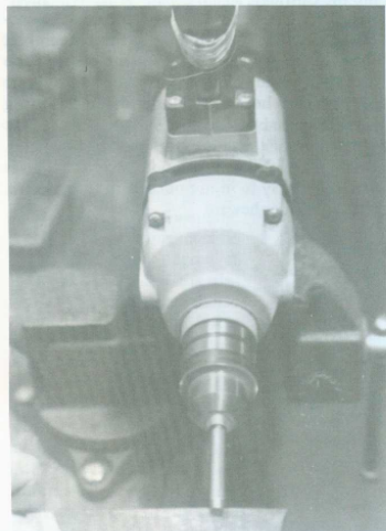
Wrap tape around bolt threads and chuck into fastened-down 1/2" drill. Work the end down to 1/16" for the firing pin.
