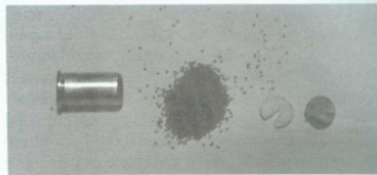
Factory original .38 propellant cartridge pulled from 40mm practice round. Load contains 6 grains of gray flake powder.
