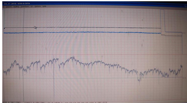
Fig.3 The changes of rotation vector of «Field Hyroscope» during Mirrors forecasting Apr.,28
