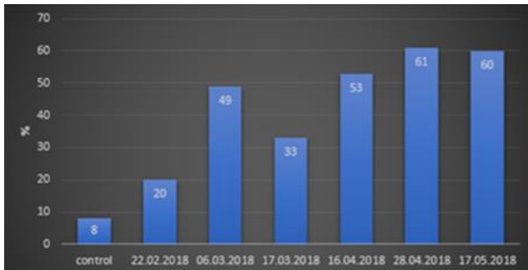
Fig.1 The number (%) of correct forecasts for further dates of earthquakes into «Kozyrev's Mirrors» using holographic treated water and at background control (according to T.Kuznetsova data)
